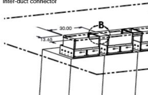
Detail B Inter-duct connector
