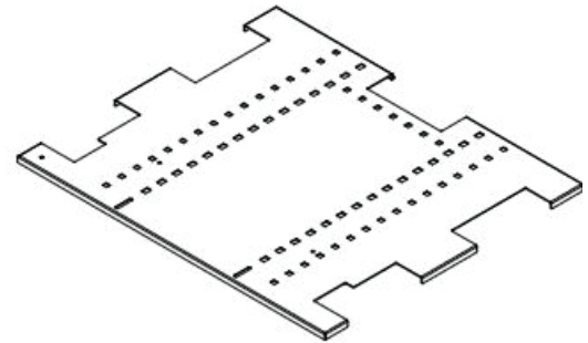
Example of a top panel designed to fit a custom rack
